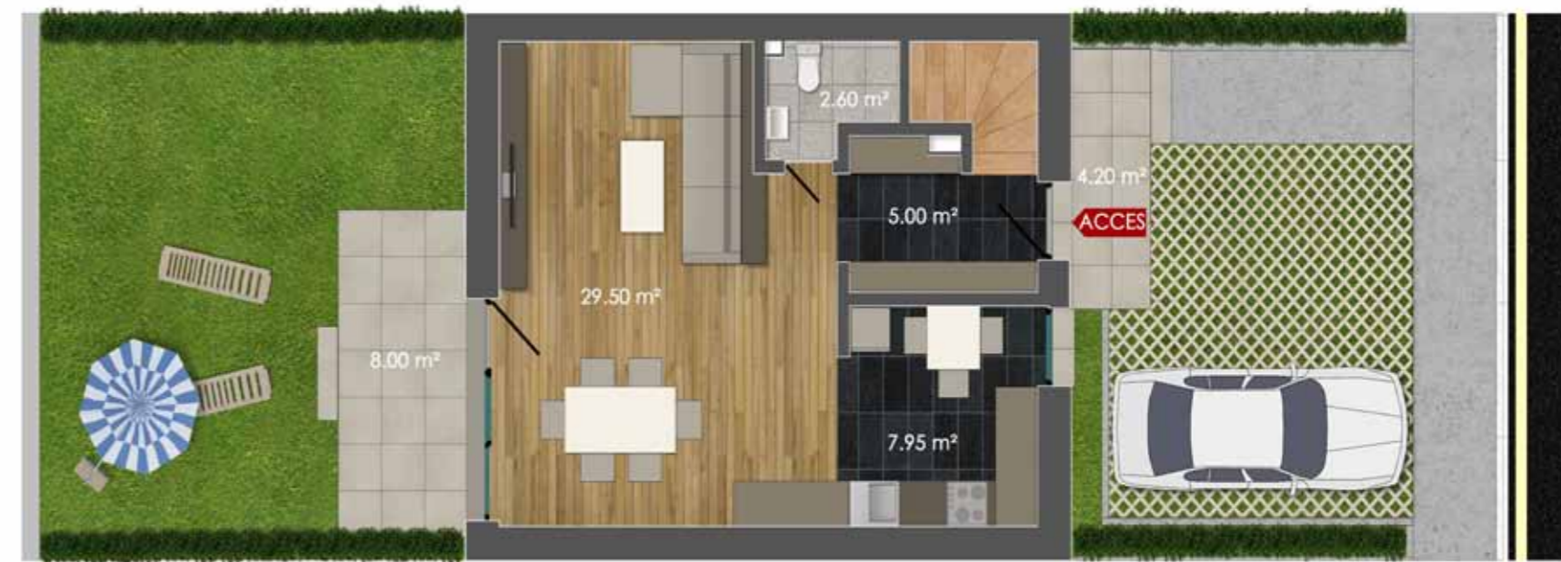
Plan parter
